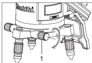
1: Fine-adjustment knob
